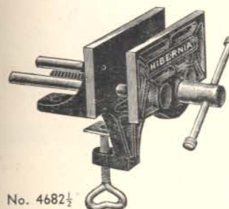
HOUSEHOLD PATTERN VICE To Clamp under Bench or Table Width of Jaws 6". Jaws Open 4 1/2". Approx. Weight - 7 lbs. Clamps to any Table Thickness to 2 1/2". Price - 7/6 each.
