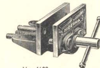
JOINERS' PATTERN VICE to Screw under Bench. Width of Jaws 6". Jaws Open 4 1/2". Approx. Weight - 5 1/2 lbs. Price 6/6 each.
